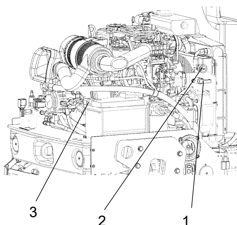
Afb. Accuruimte 1. Accu-isolator (alleen in versie PLUS) 2. Stopcontact, 12V 3. Kabelschoen
