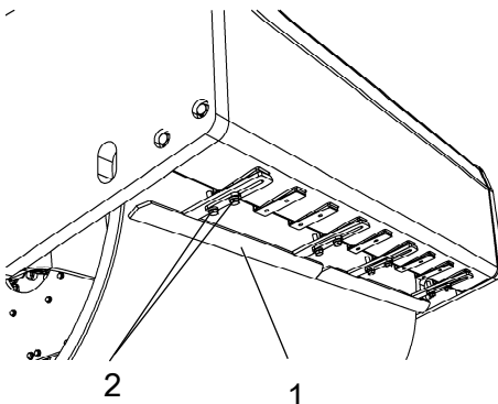
Fig. Racleur (CA1400 D)
