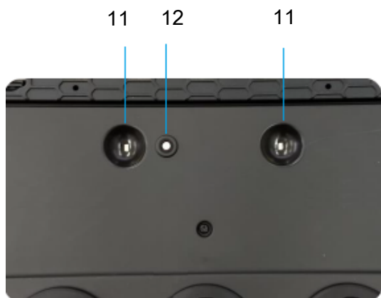
Fig. Voyants LED 11. Voyants LED 12. Contact
