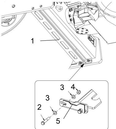
Fig. Racleur (CA1300 D)
