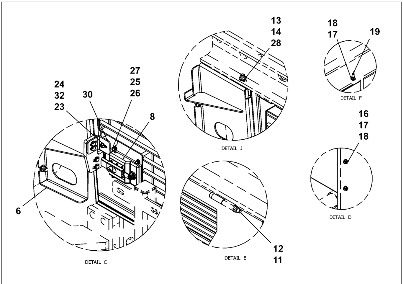
4812221194 Side doors
