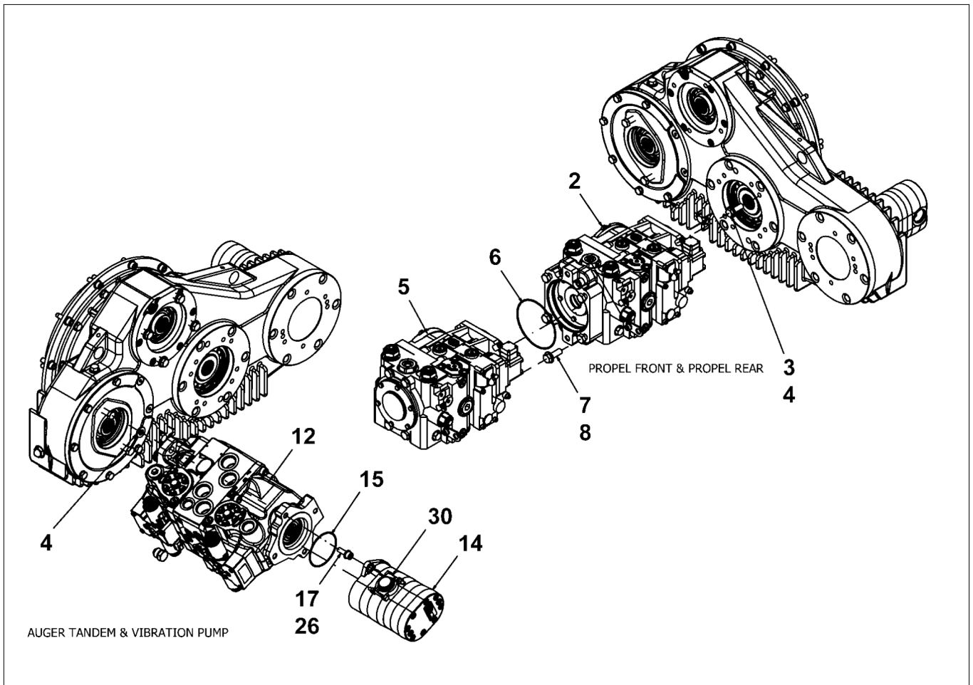
4812200024 Pump drive
