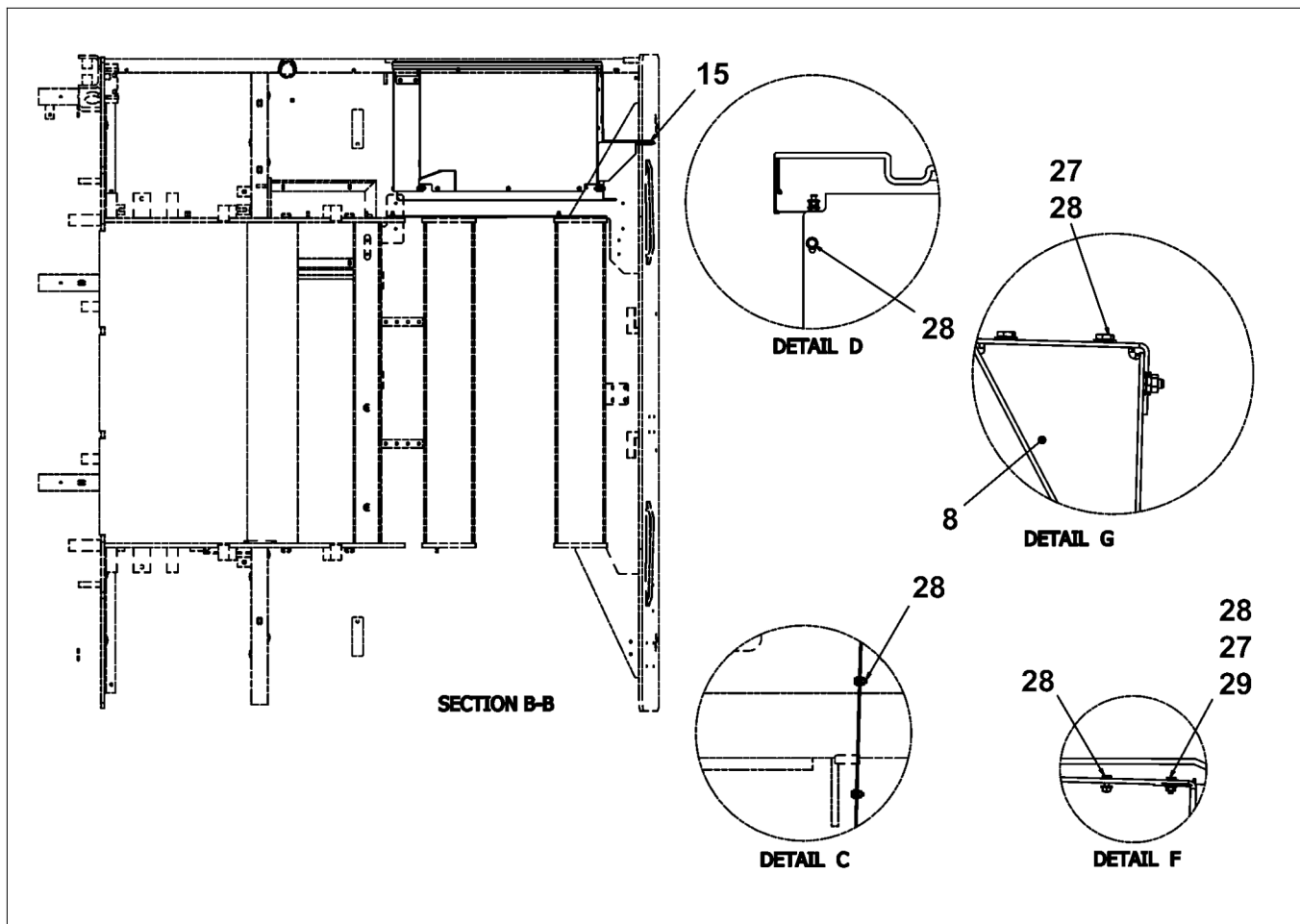
4812222361 Cooler shroud
