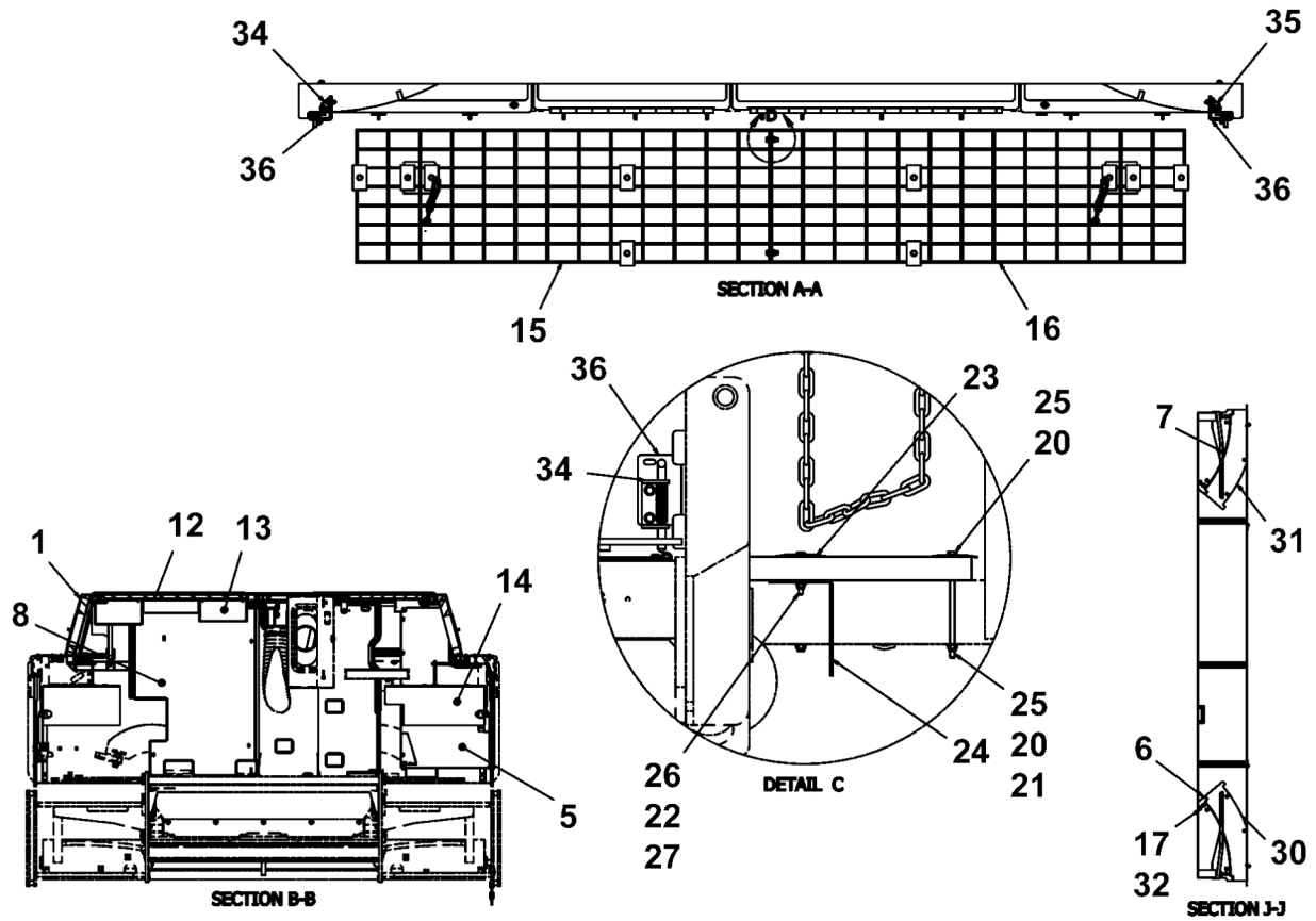
4812200022 Platform assembly
