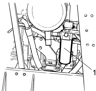
Fig. Motorrum 2. Hydrauloljefilter (2st).
