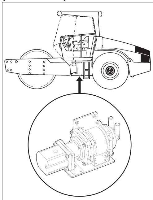
Afb. 50 Compressor
