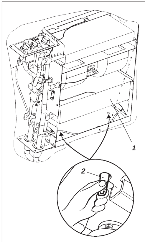
Afb. 49 Airconditioning 1. Koelelement 2. Aftapklep (x2)
