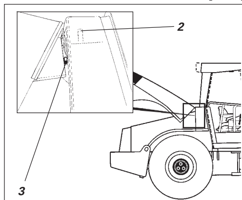
Fig. 41 Hydraulikkoljetank
