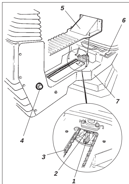
Fig. 40 Stollager
