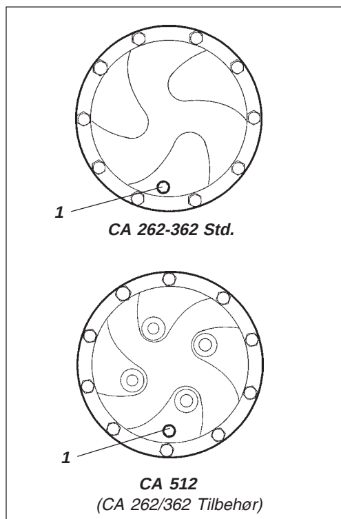
Fig. 47 Planetgir/stilling for avtapping 1. Plugg
