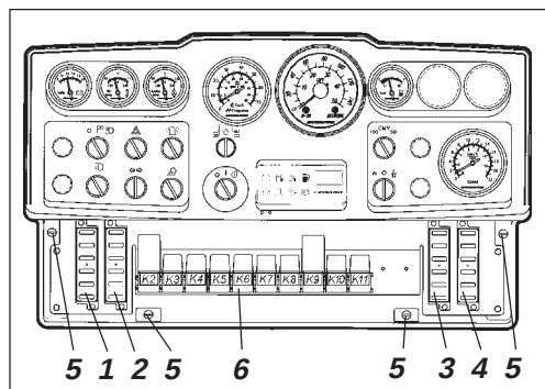
Fig. 61 Instrumentpanel
