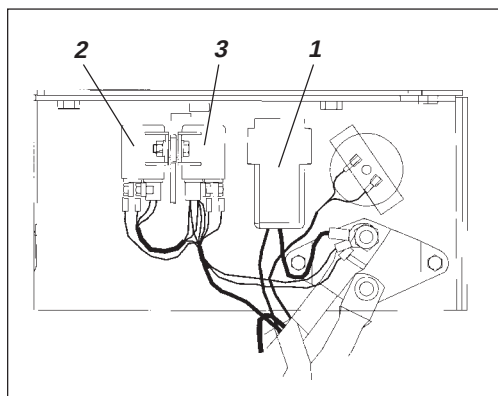
Fig. 53 Motorrum (Cummins steg 1 motor)
