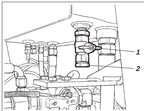
Fig. 35 Hydraultank undersida
