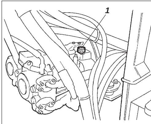
Afb. 20 Pompoverbrenging 1. Peilstok
