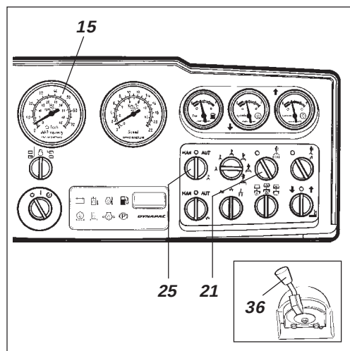
Fig. 18 Instrumentpanel
