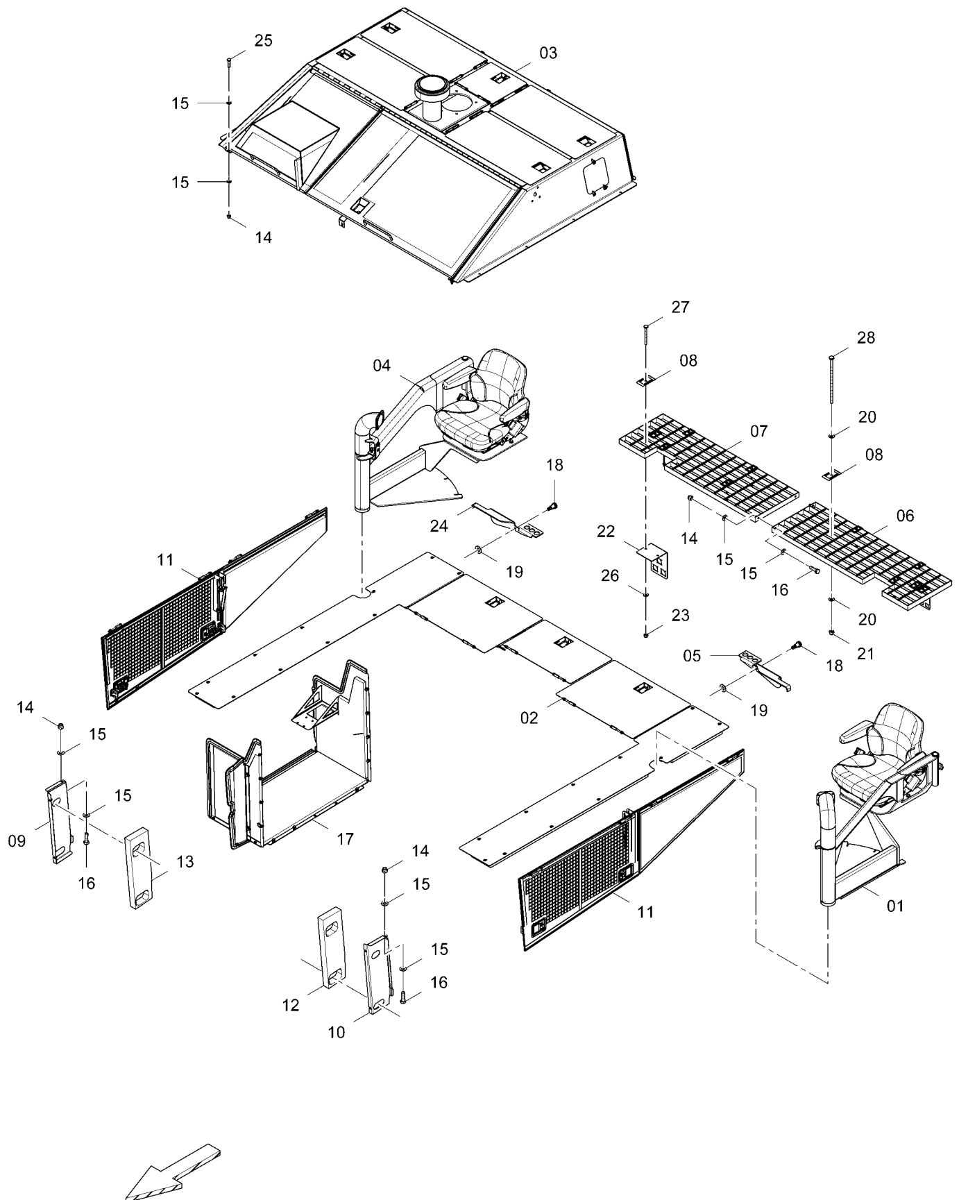
D717110000 Platform 2
