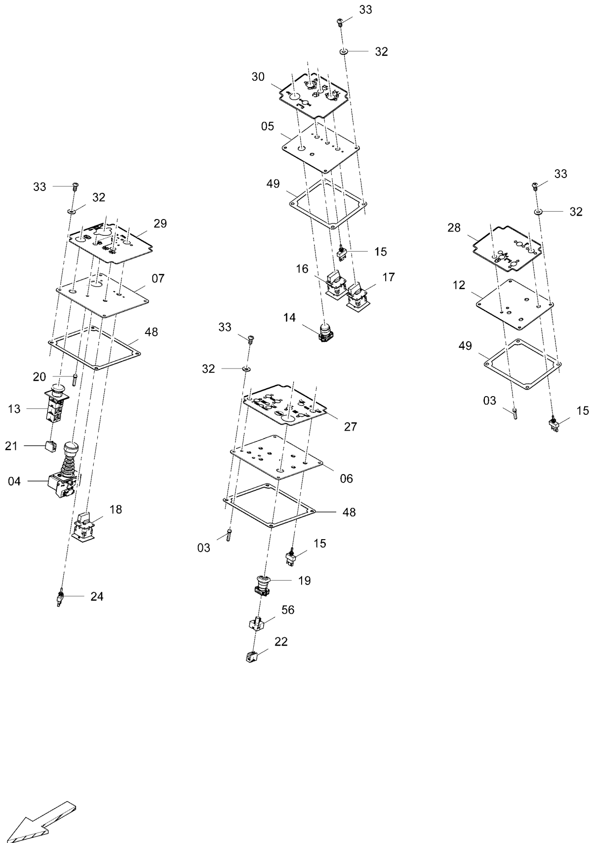
D717103500 Operator console rh
