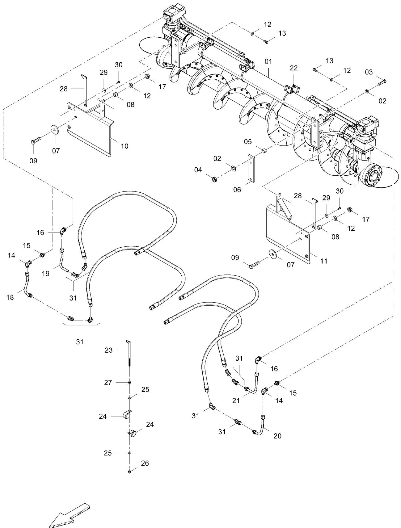
D717180001 Auger 2
