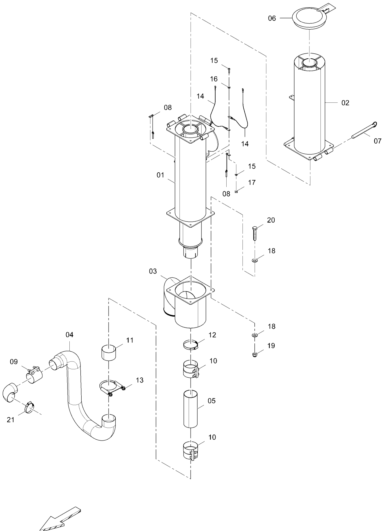
D717081500 Muffler, 10` drive complete
