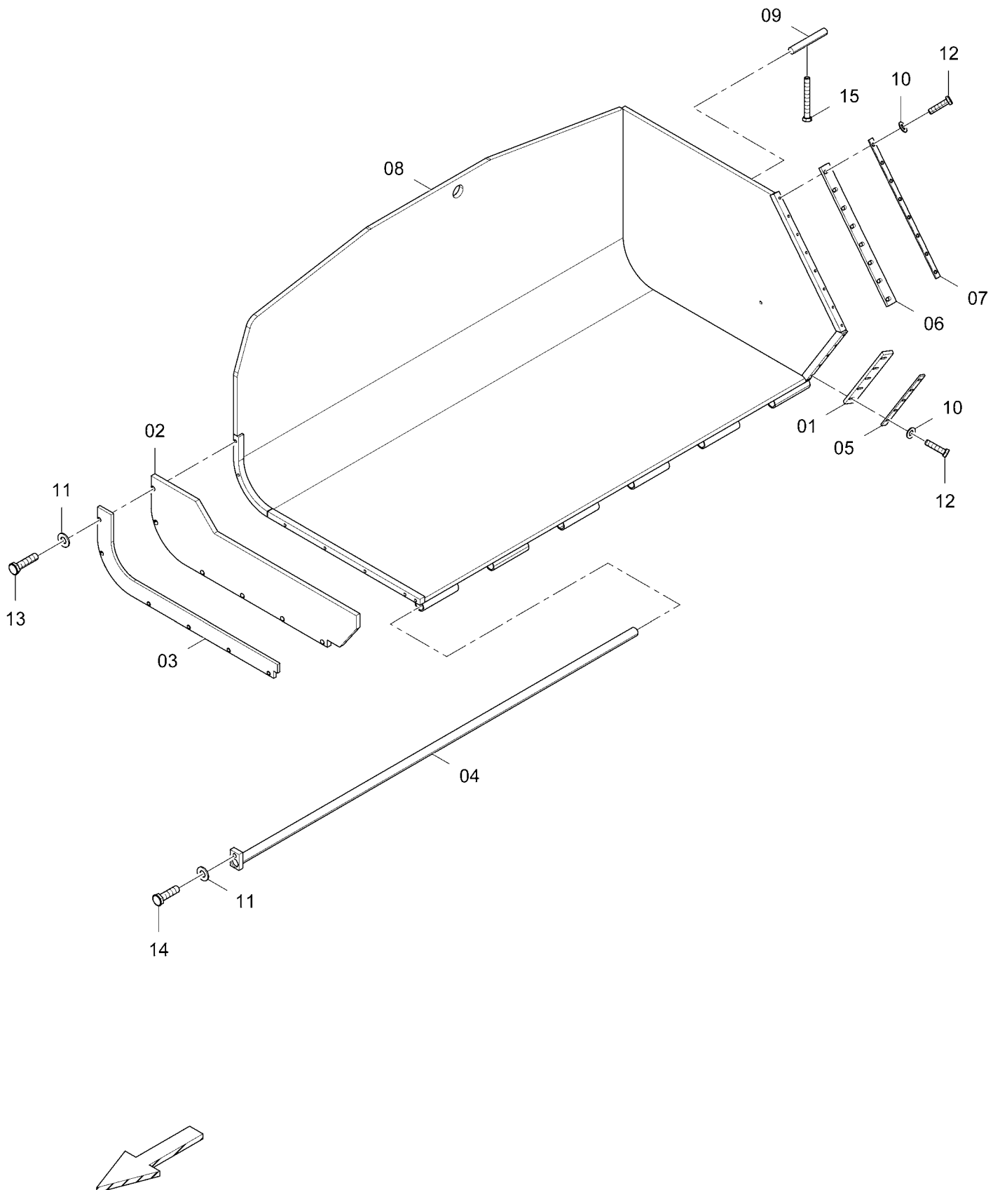
D717071000 Hopper Assembly, right side, 10 ft.
