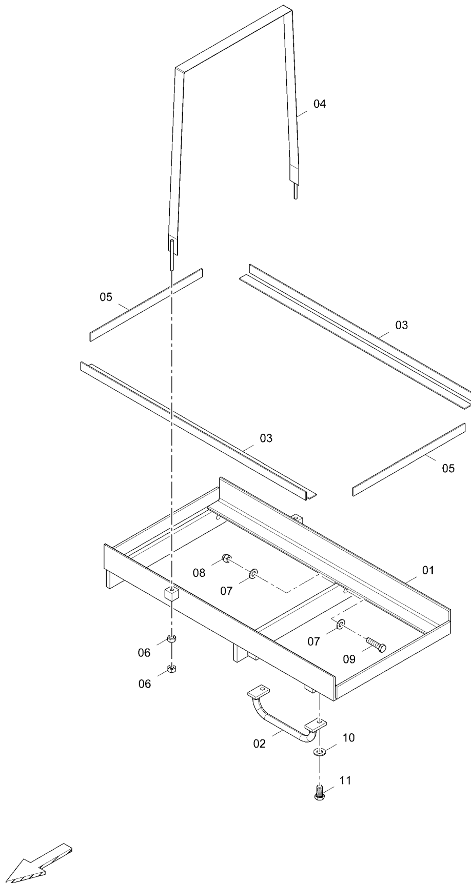
D717083000 Bracket assembly, hydraulik tank
