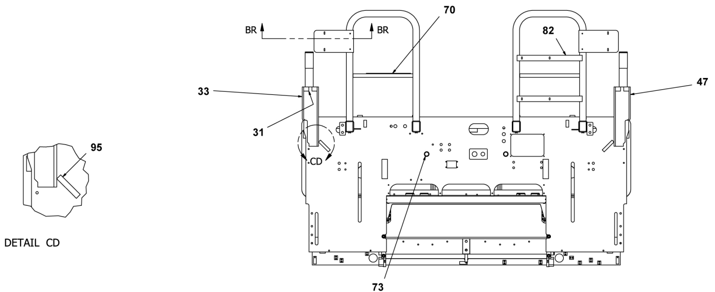
D717010500 frame, main
