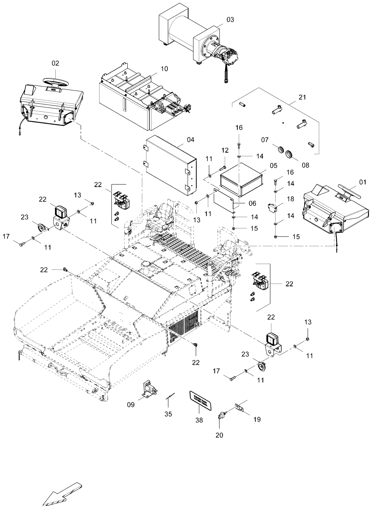
D717100000 Electrical system 2
