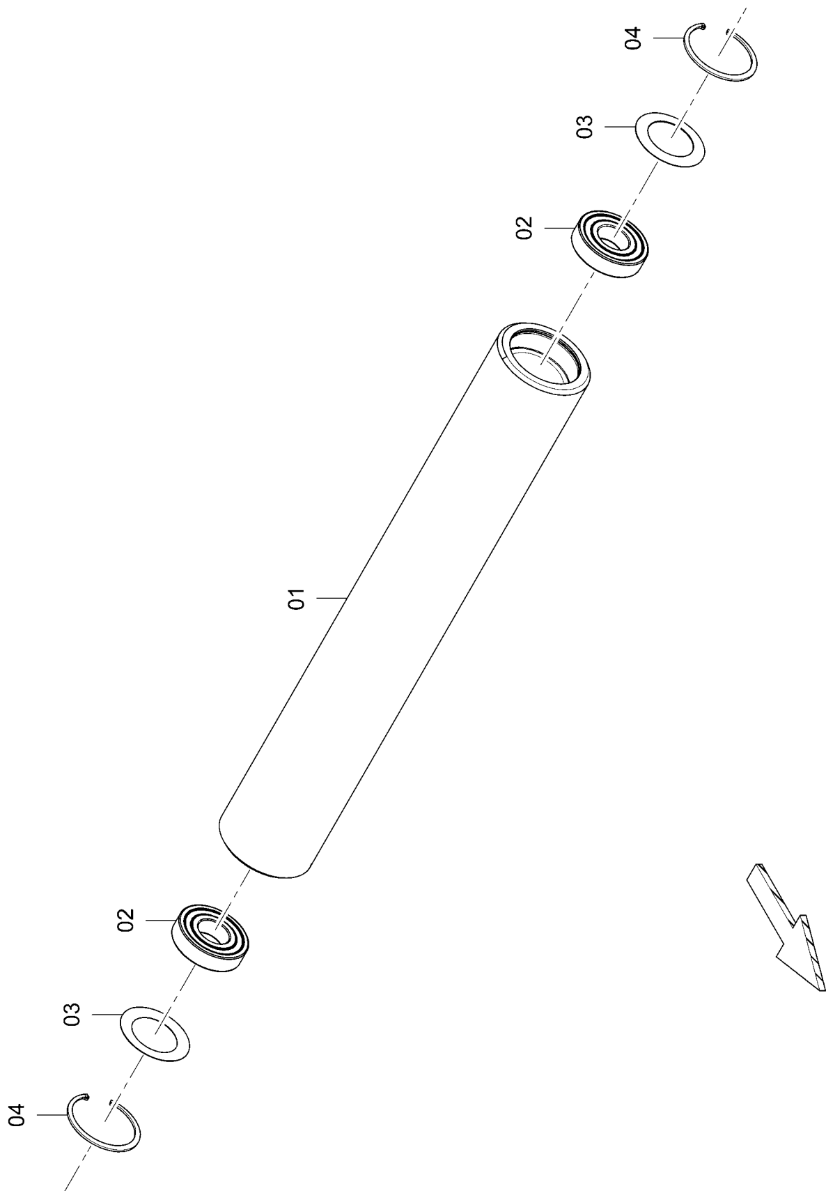
D717011005 Roller
