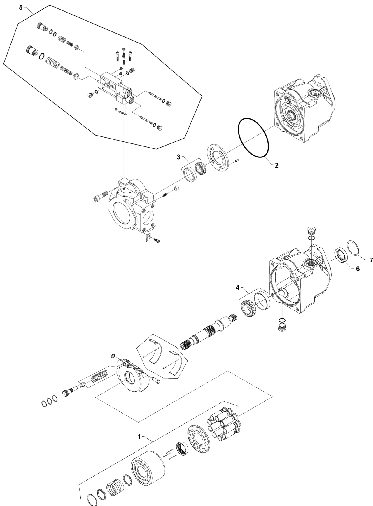
D717194500 Pump, conveyor / work
