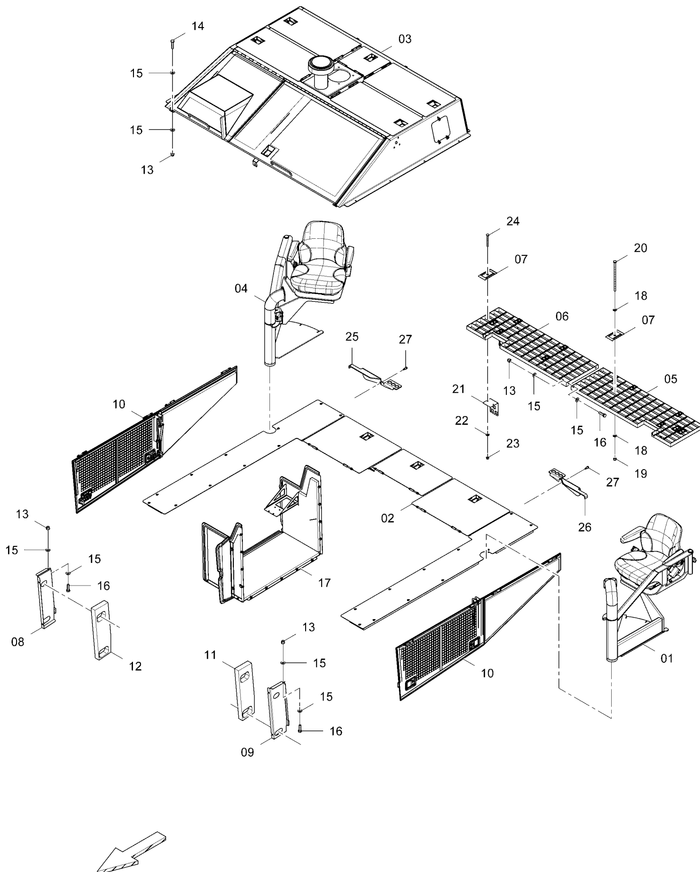
D717110000 Platform 3
