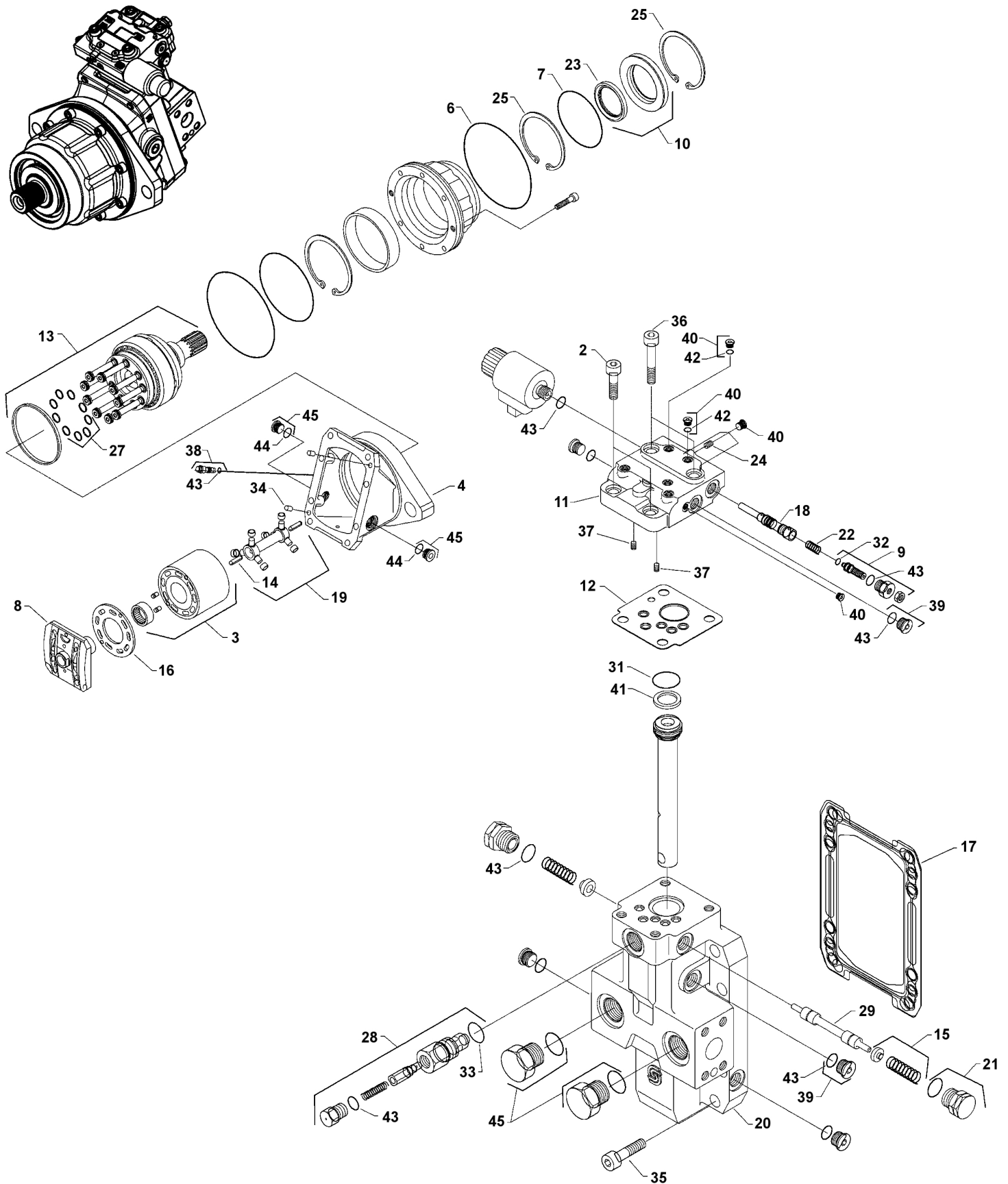
D717171014 Motor Track assy
