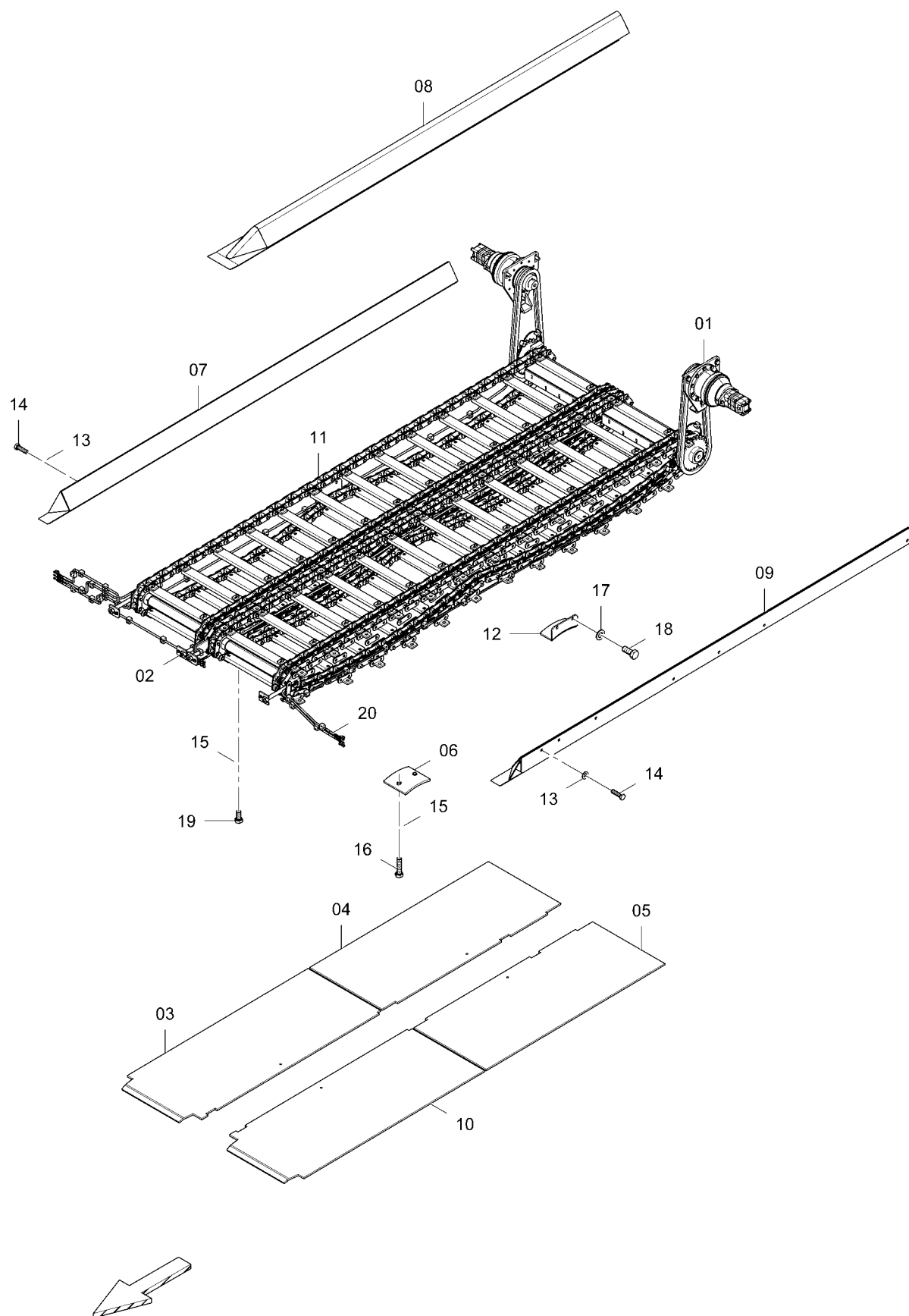
D717060000 Conveyor 2
