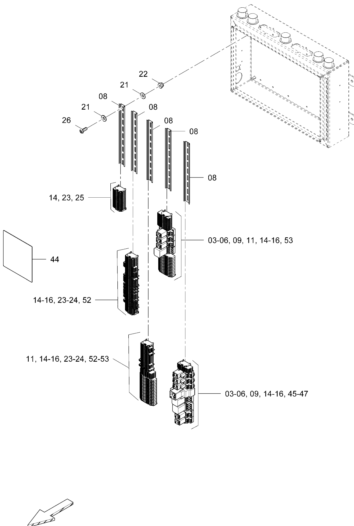
D717104000 Dc control panel
