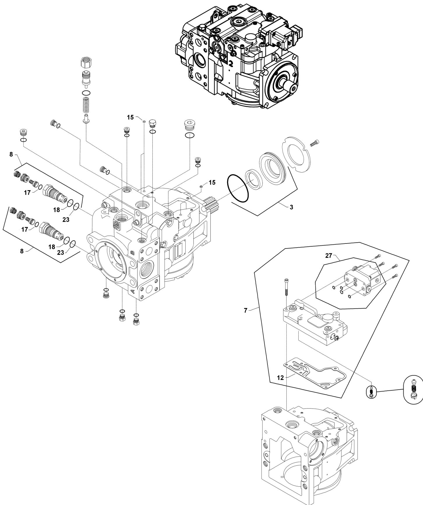
D717193500 Pump, generator
