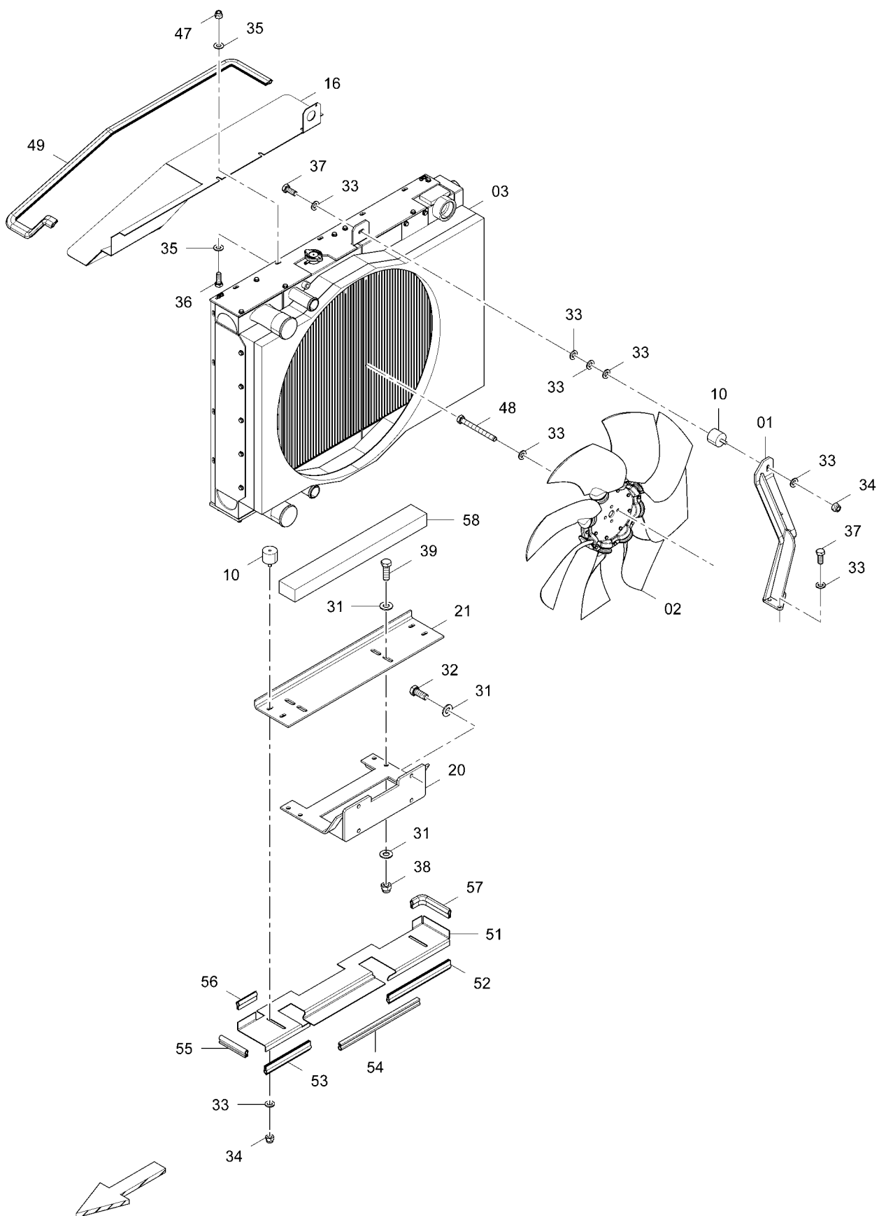
D717085000 Installation, water-oil-air cooler 2
