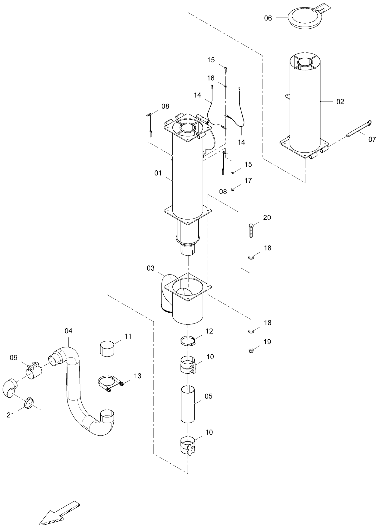
D717081500 Muffler, 10` drive complete 00A
