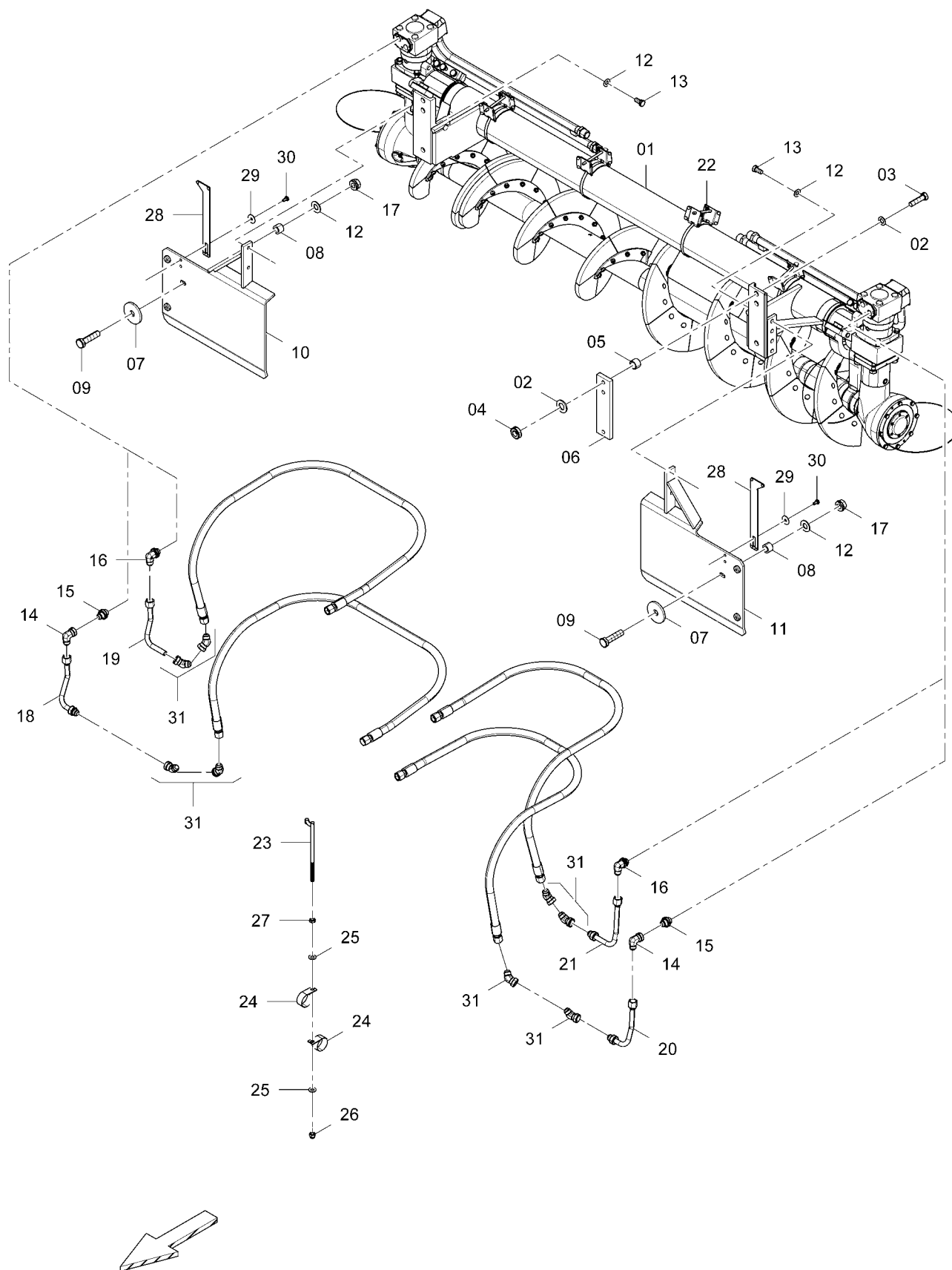
D717180001 Auger 2
