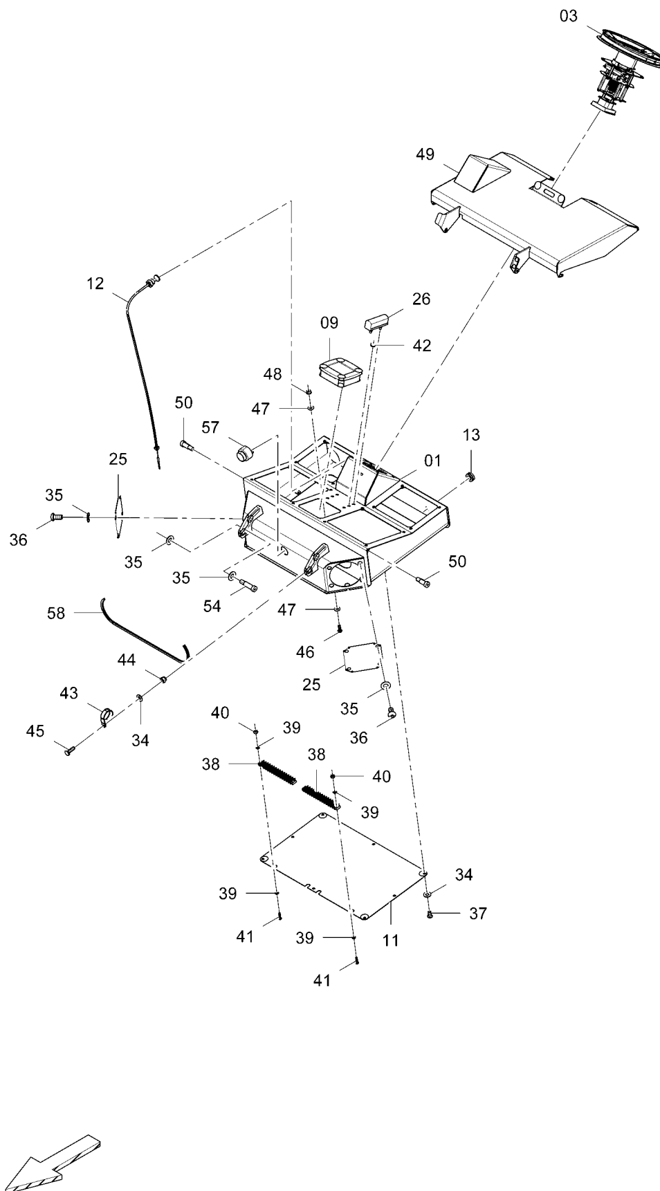
D717103000 Operator console lh
