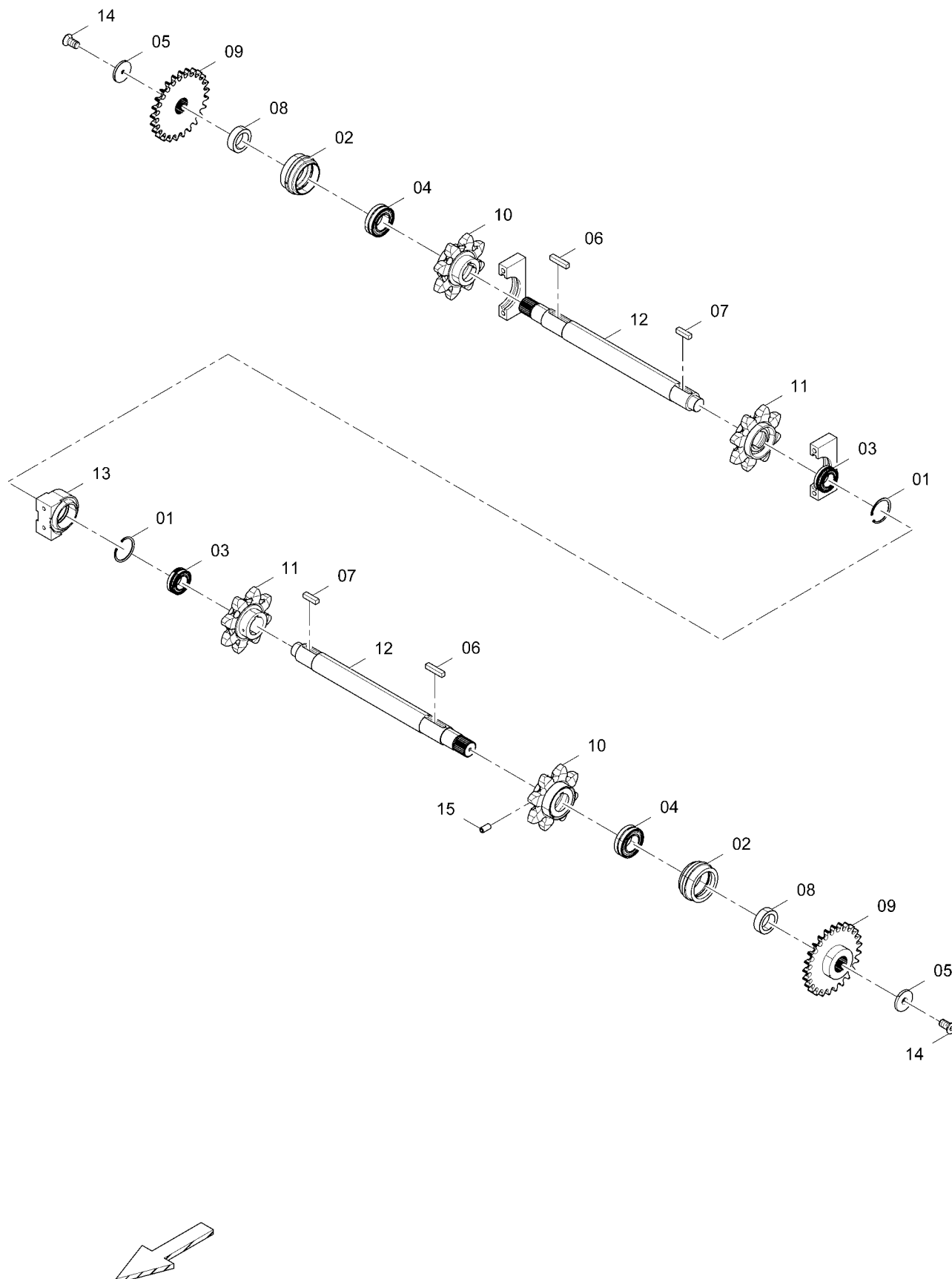
D717061018 Drive, conveyor 3
