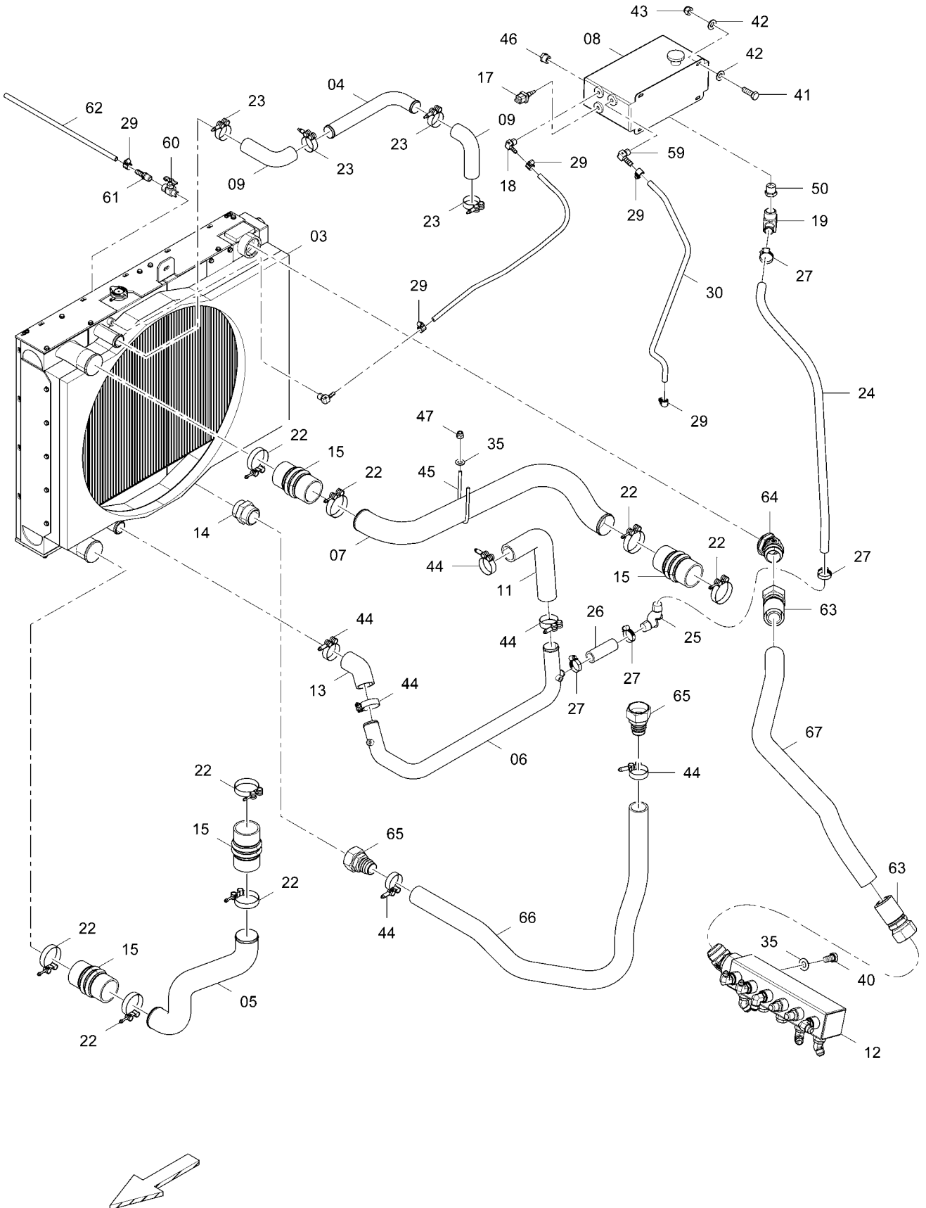
D717085000 Installation, water-oil-air cooler 2
