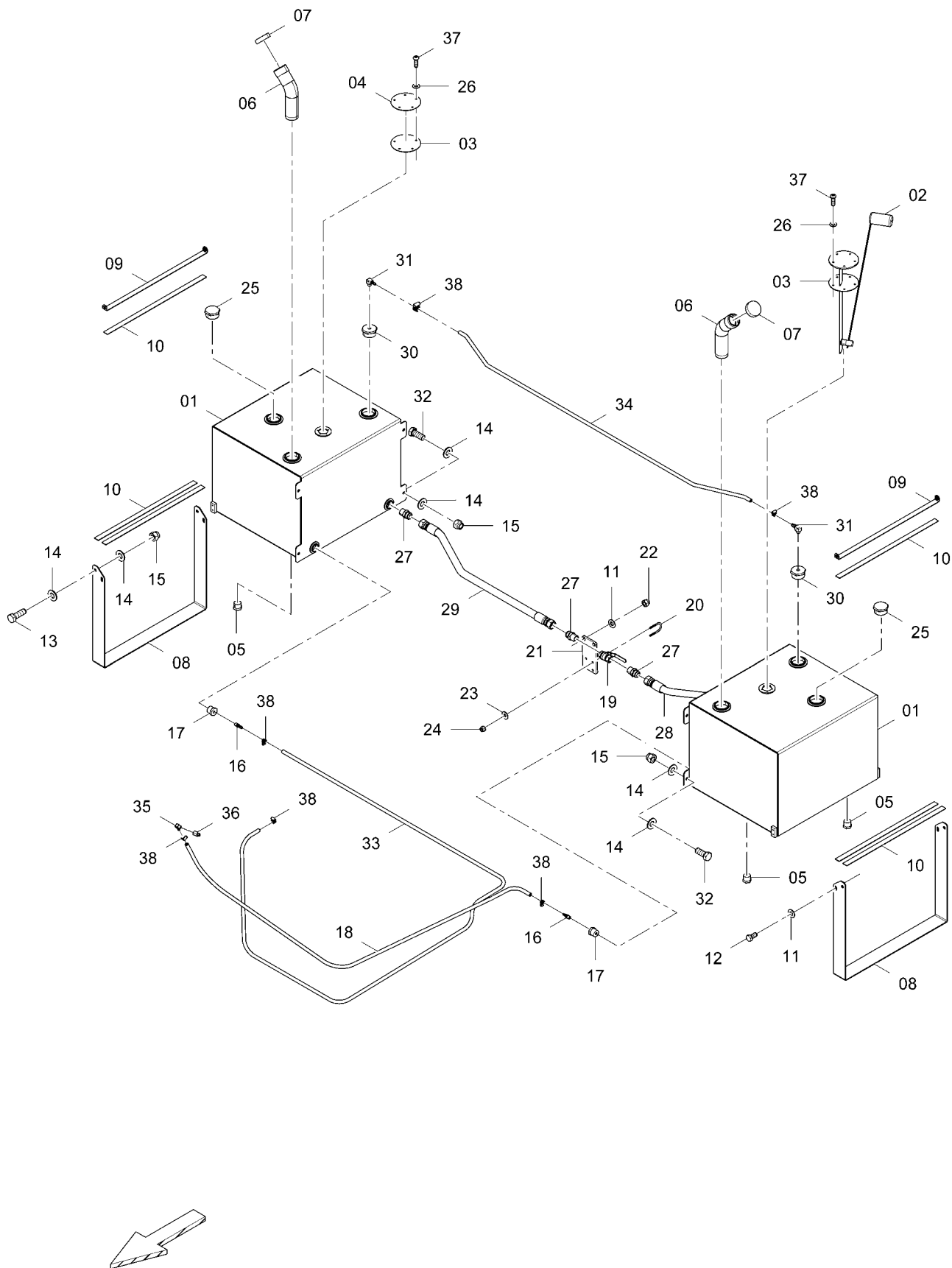
D717083500 Fuel tank 00B
