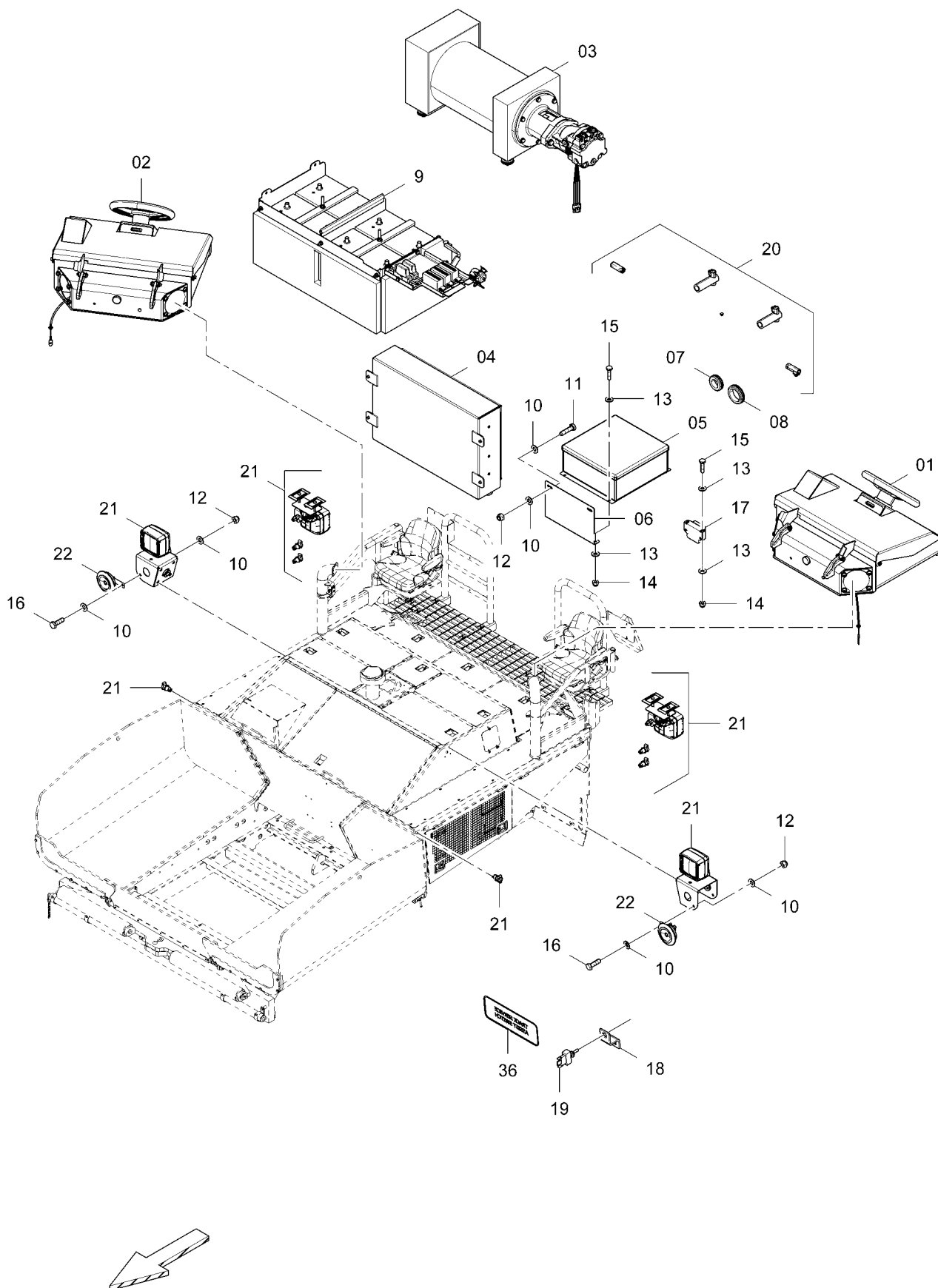
D717100000 Electrical system 3
