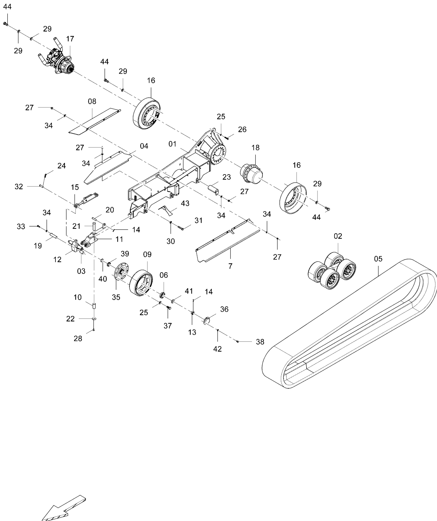
D717170500 Track left
