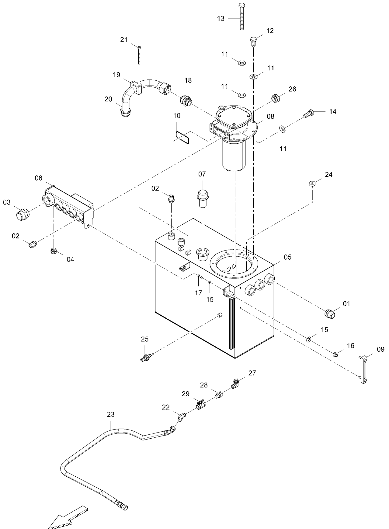
D717084500 Hydraulic tank
