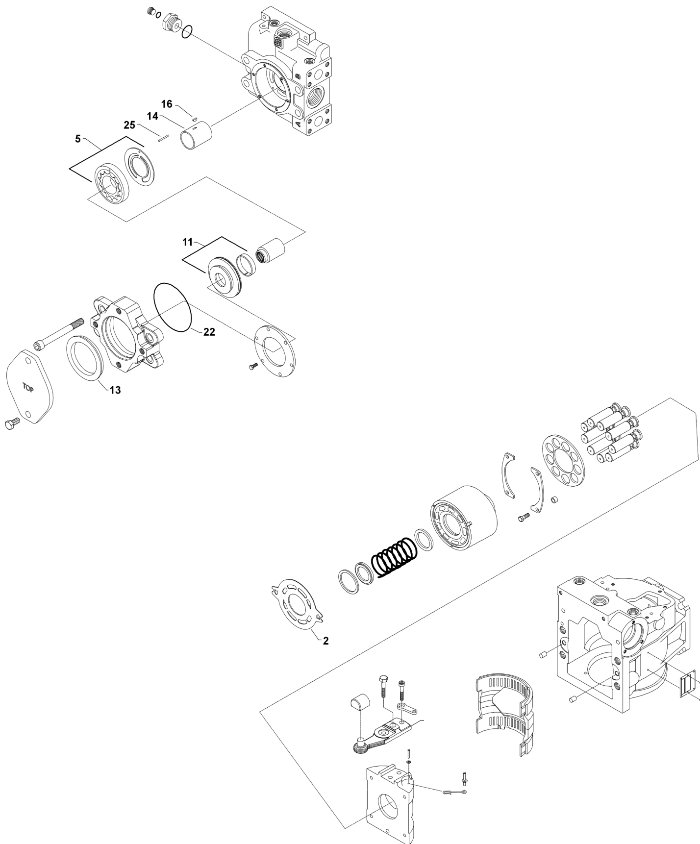
D717193500 Pump, generator
