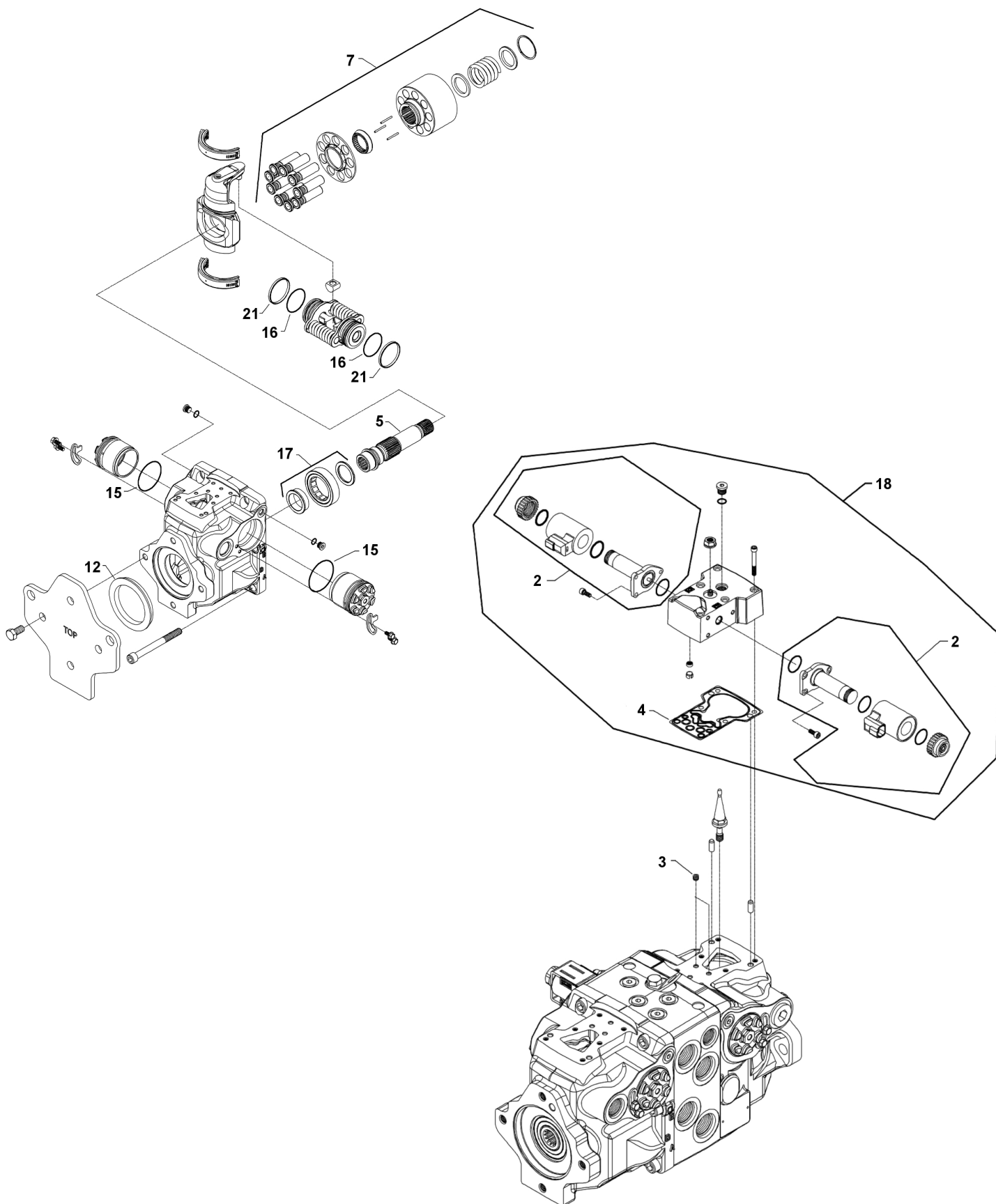
D717192500 Pump, auger tandem
