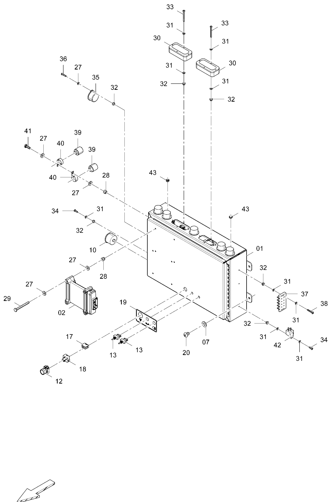
D717104000 Dc control panel
