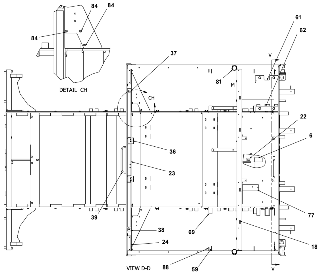
D717010500 frame, main
