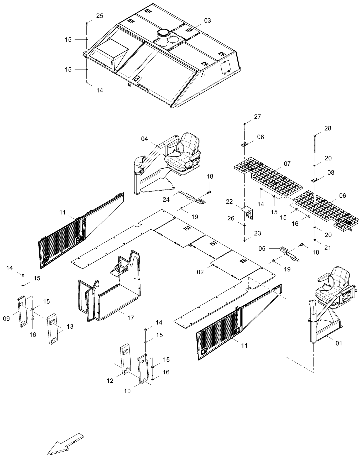
D717110000 Platform 2
