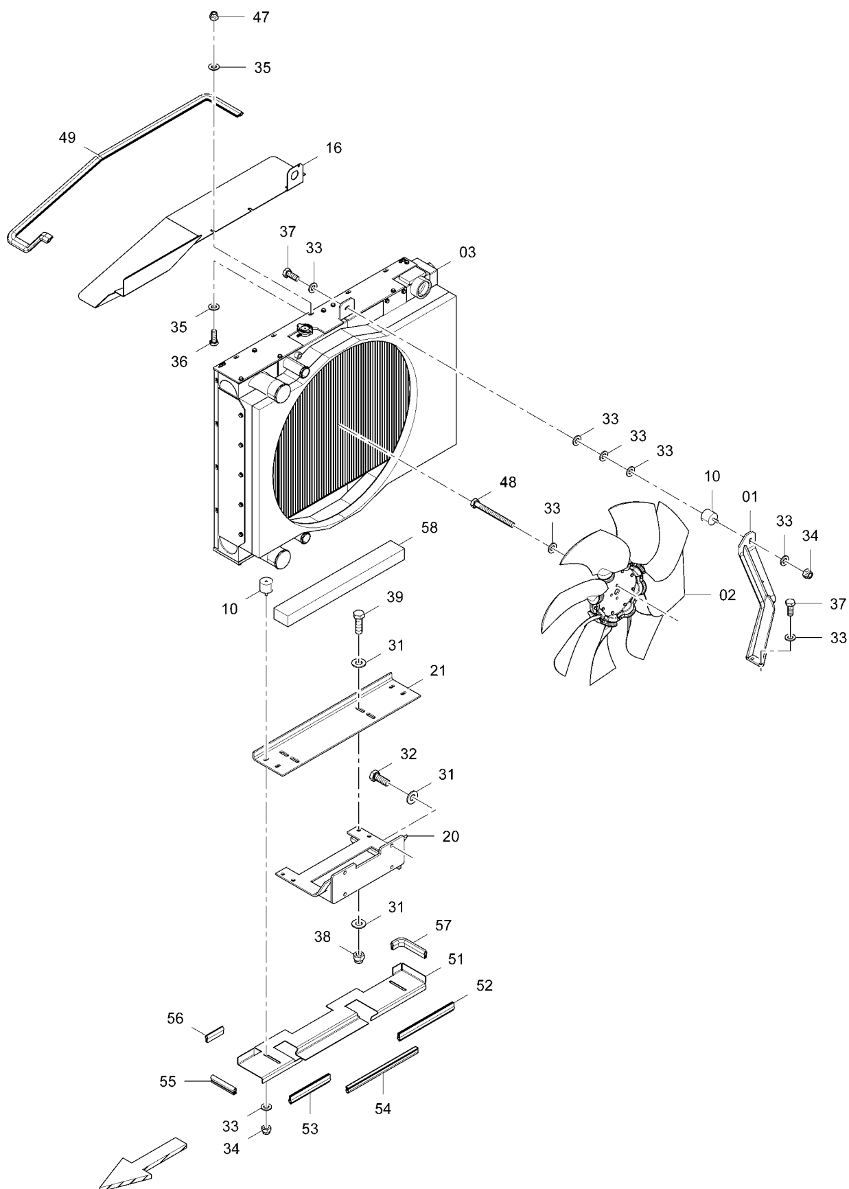
D717085000 Installation, water-oil-air cooler 3
