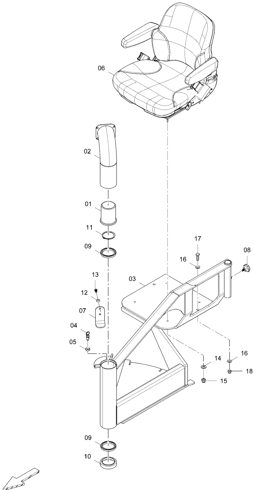
D717113000 LH Operator station
