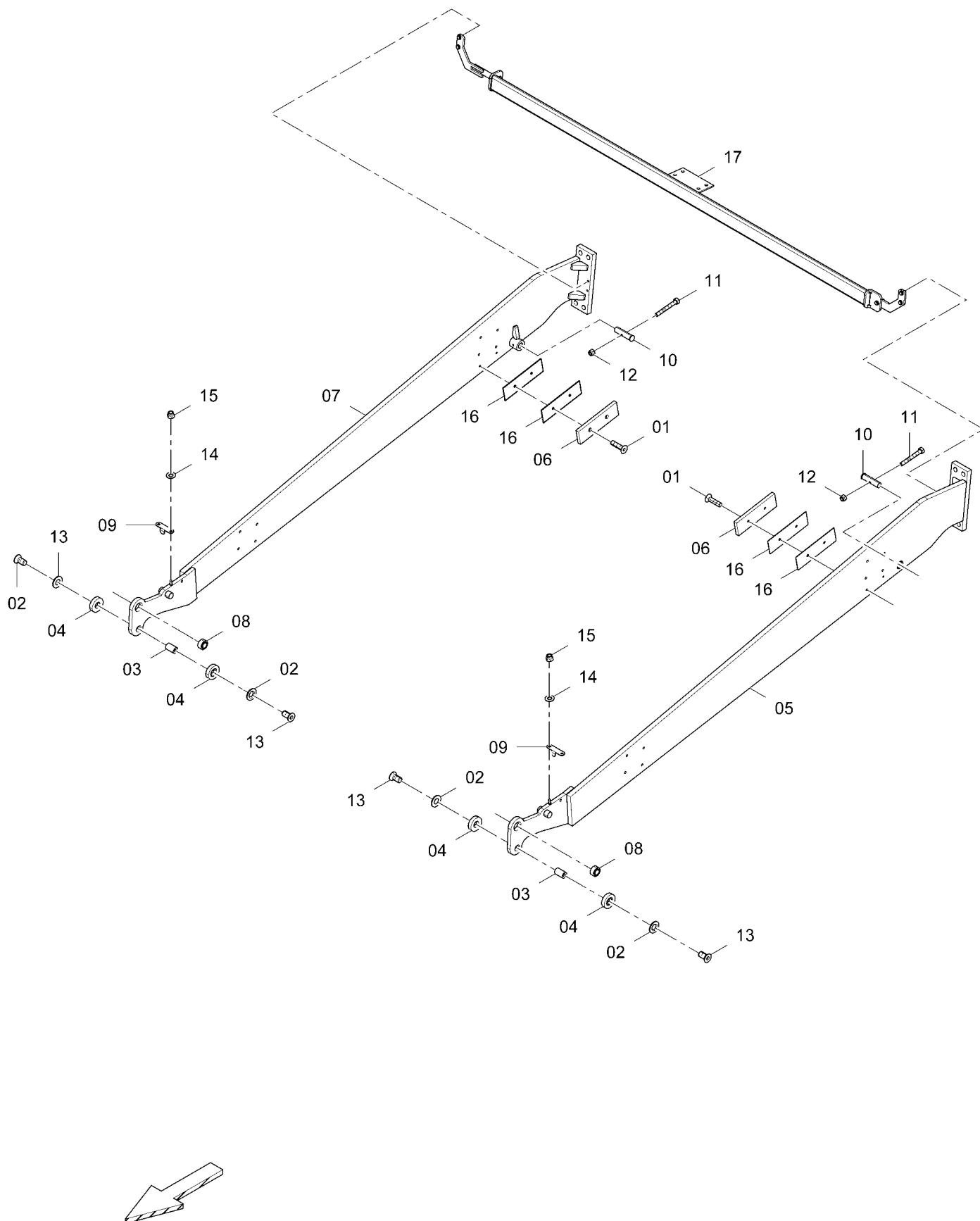
D717040000 Screed arm 2
