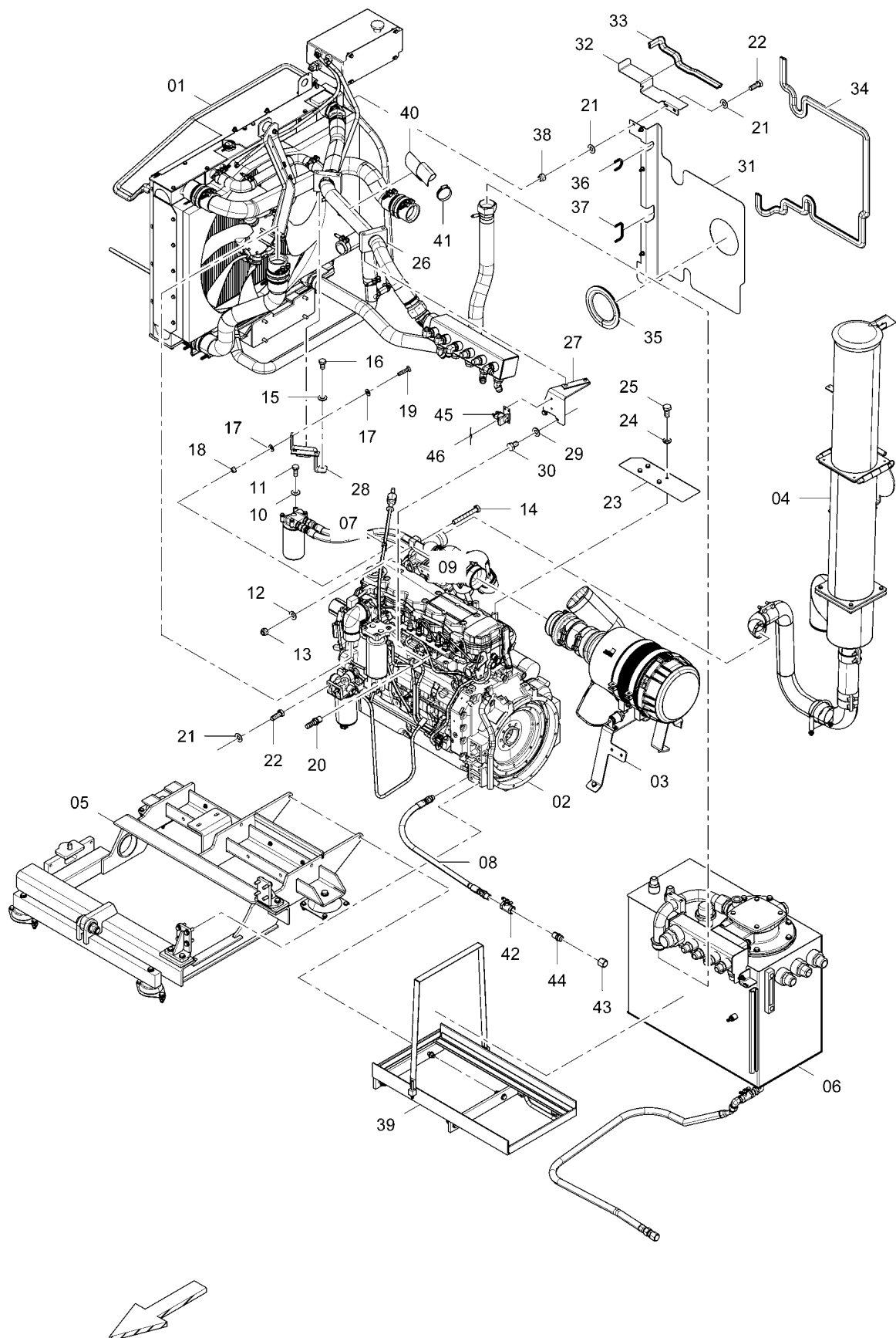
D717080000 Drive
