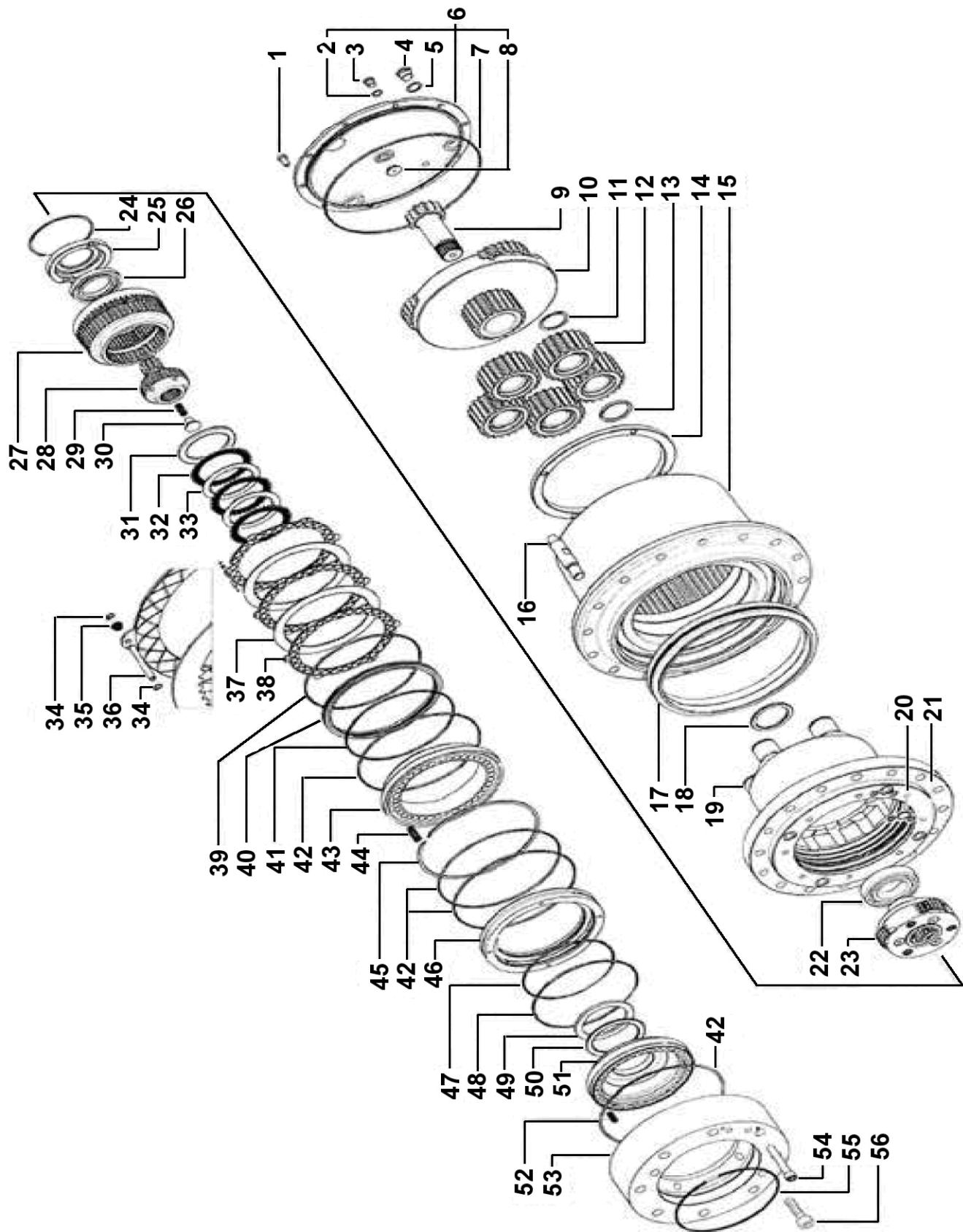
D717170600 Gearbox, Track drive
