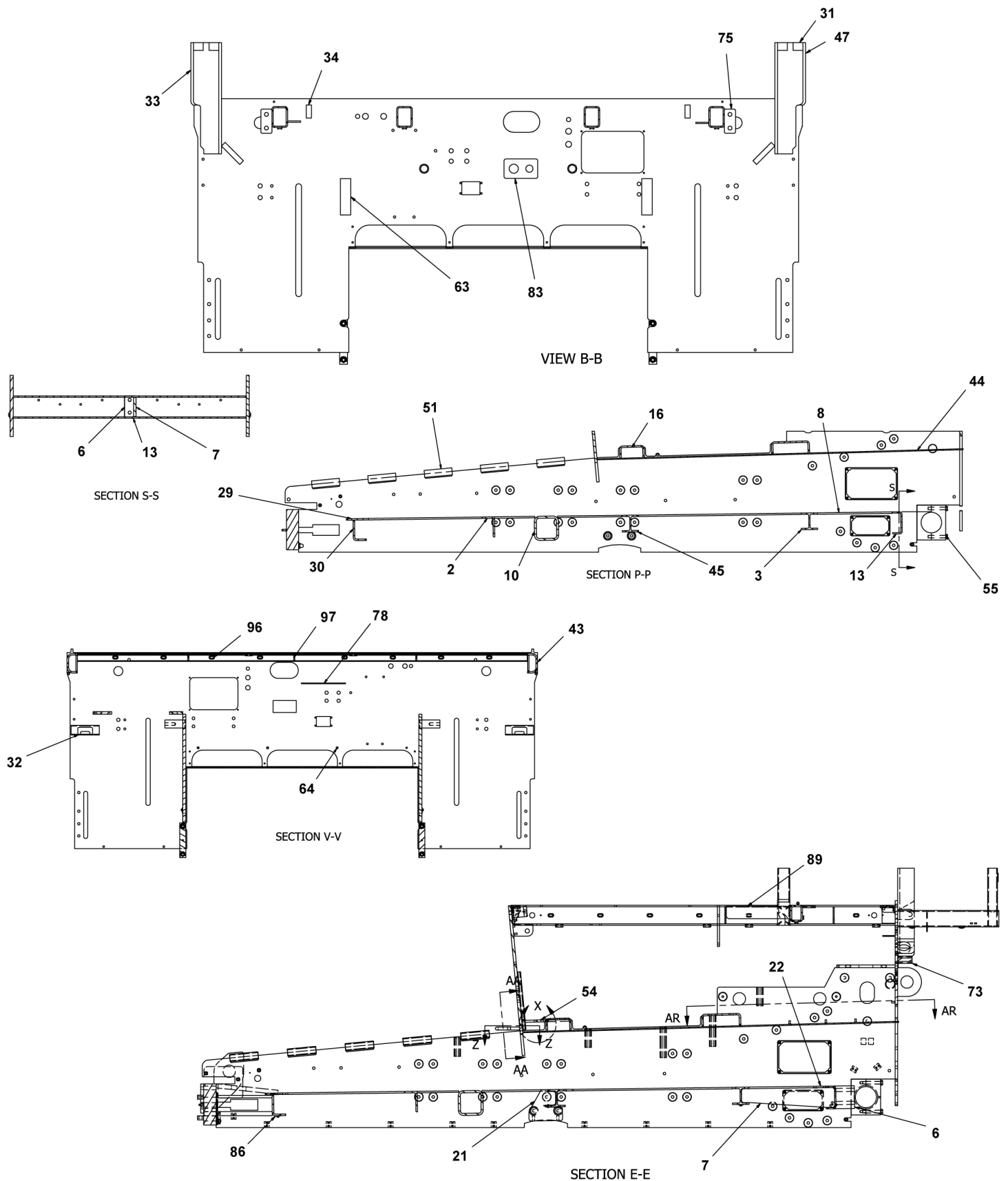
D717010500 frame, main
