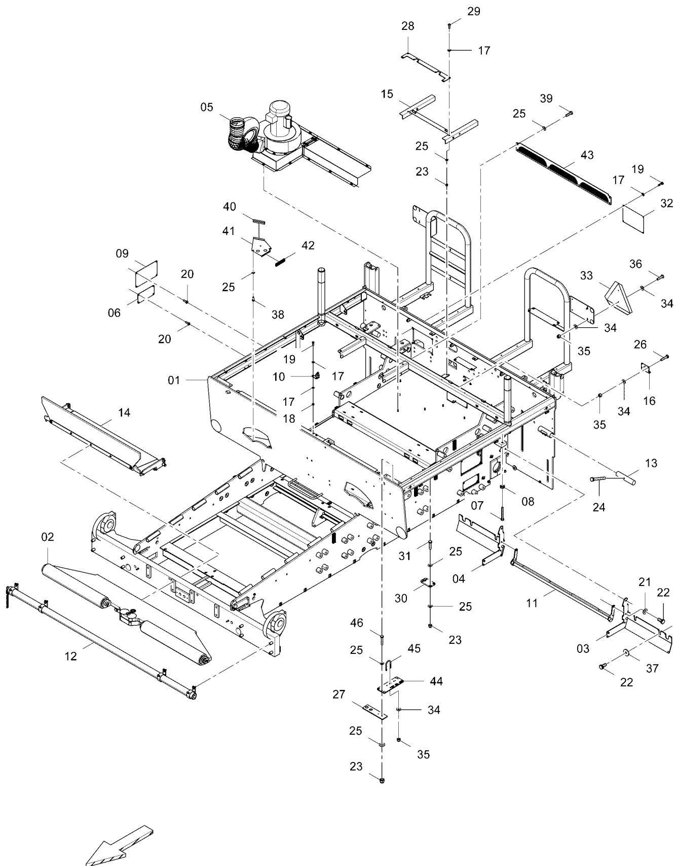
D717010000 Frame 00A
