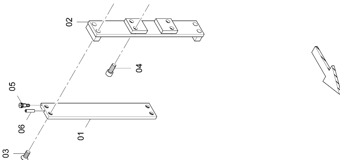
D717172001 Screed leveling guide
