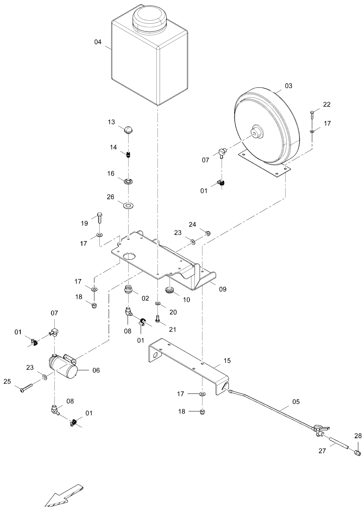
D717909500 Wash down
